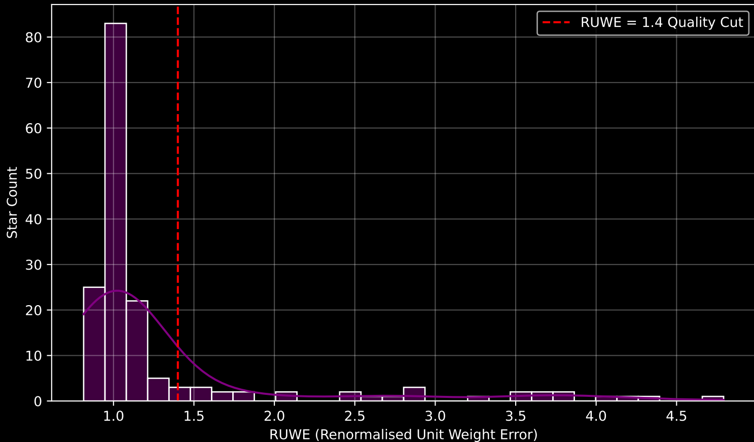
GAPOGEE DR17 Field [056+39_MGA] RUWE Distribution (n= 165)
