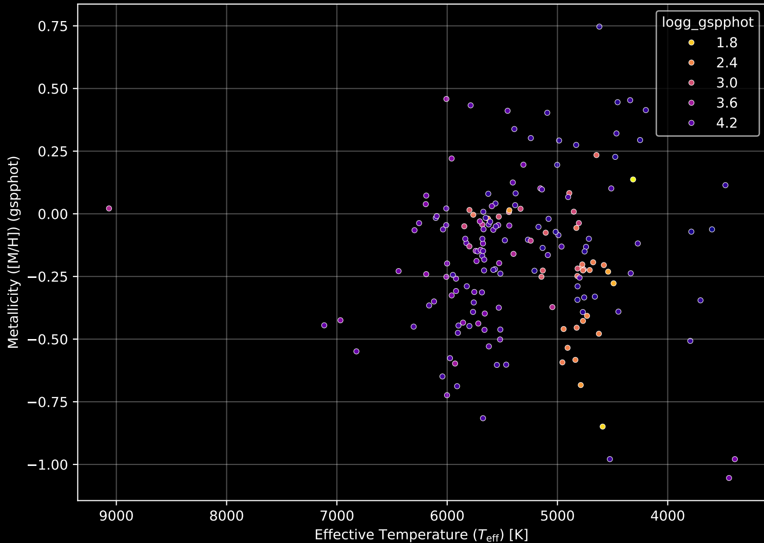
APOGEE DR17 Field: [056+39_MGA] Stellar Population Parameters (n= 175)
