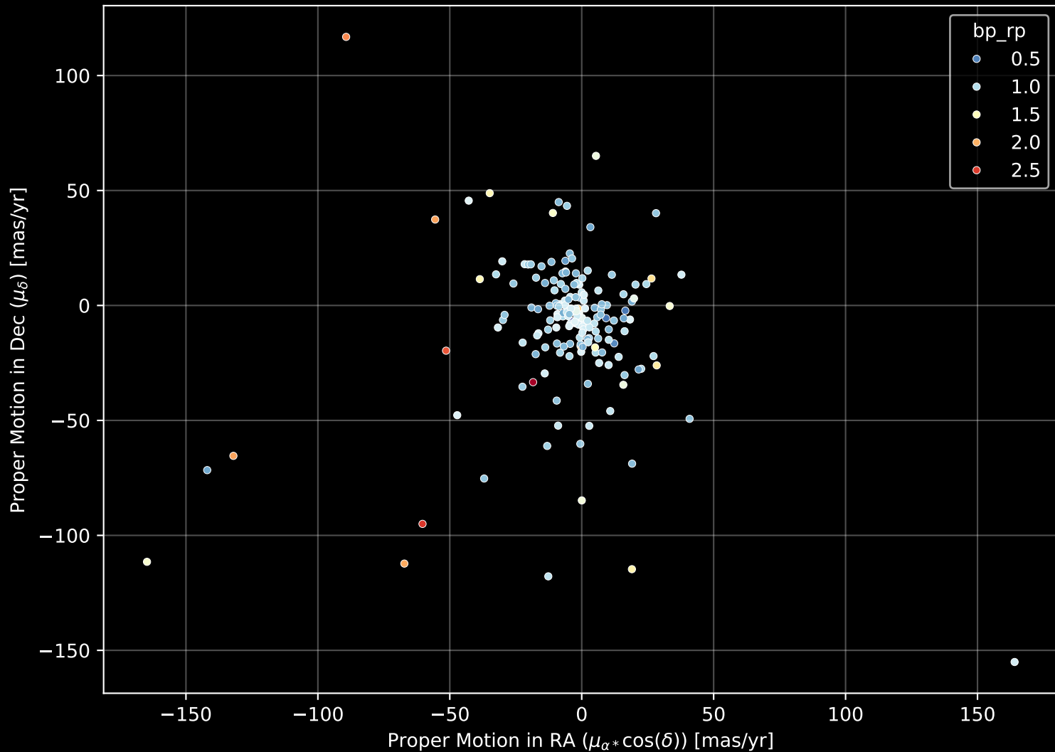
APOGEE DR17 Field: [056+39_MGA] Proper Motion Diagram (n= 175)
