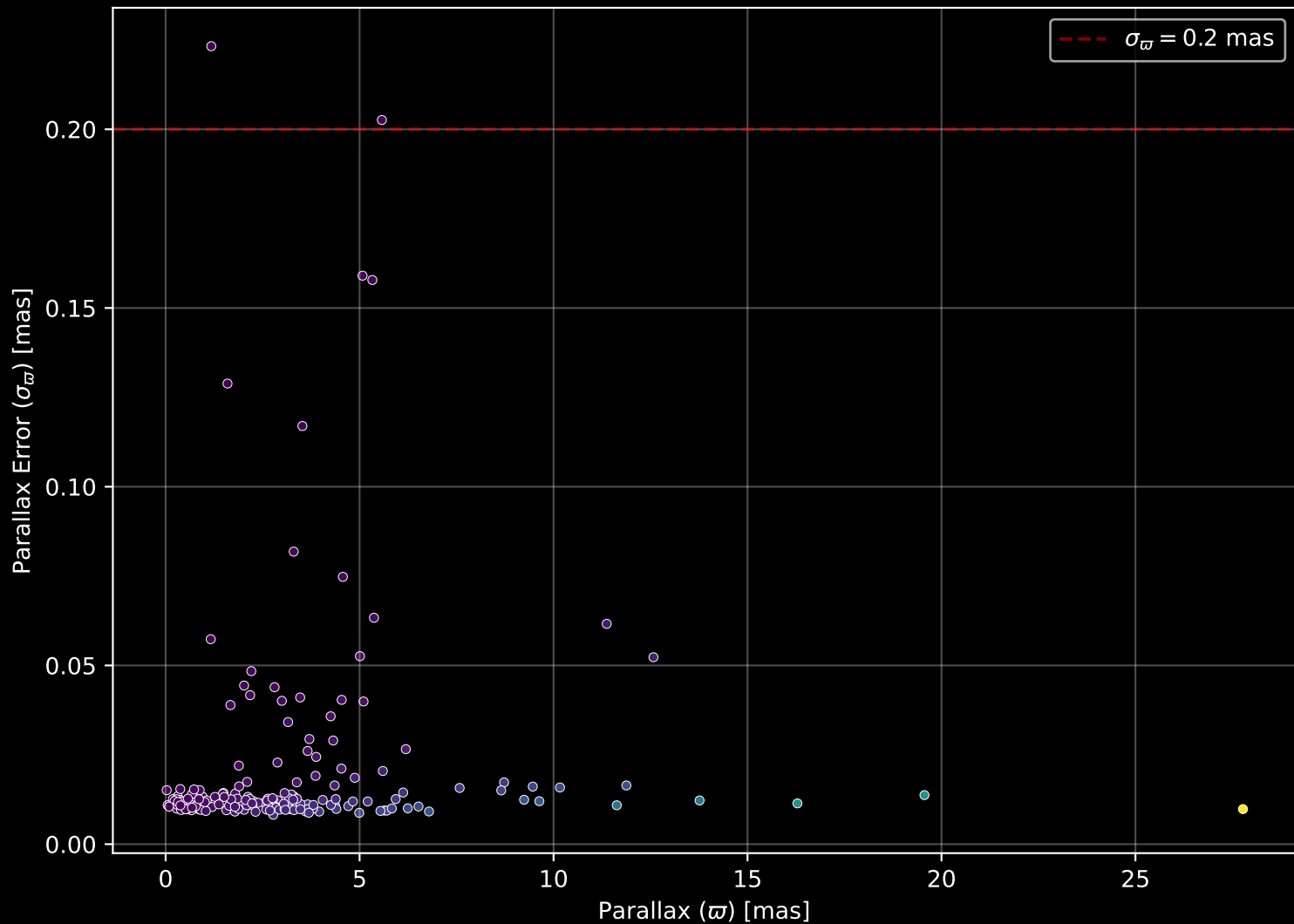
APOGEE DR17 Field: [056+39_MGA] Parallax Quality (n= 175)
