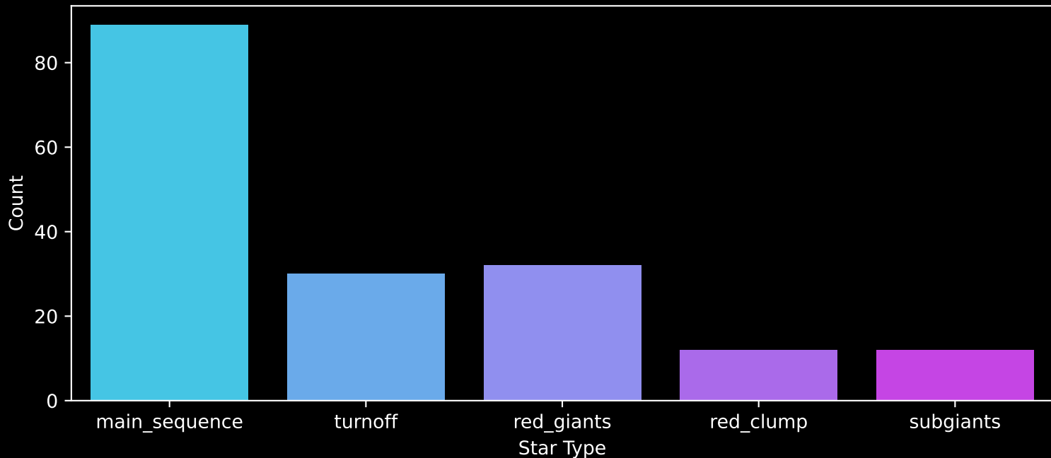
APOGEE DR17 Field: [056+39_MGA] Count plot of Star Type
